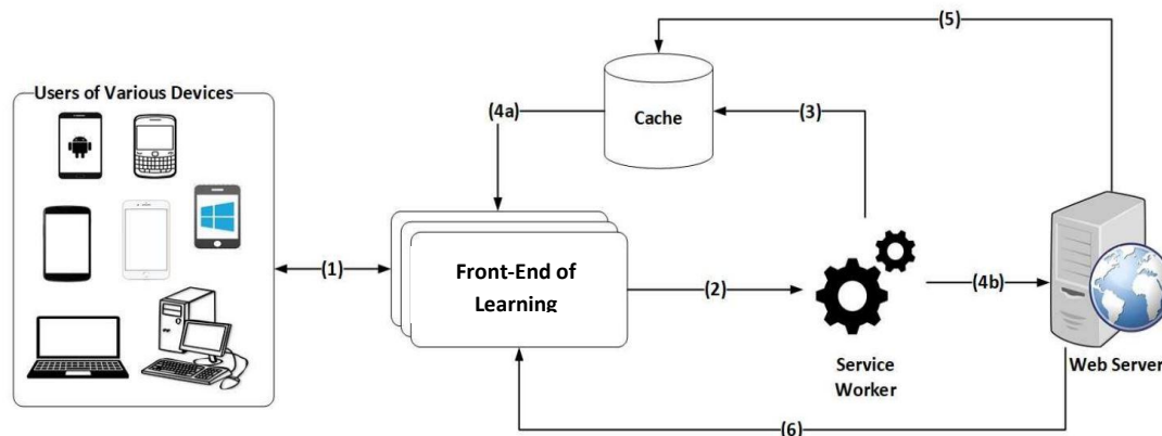
Figure 1: E-learning PWA Model (Researcher's Model)
